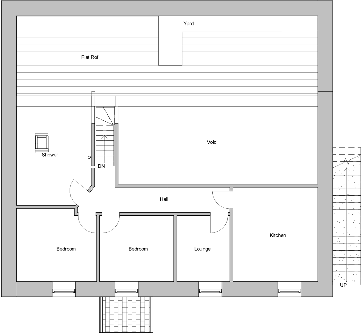
2 Existing First Floor 1 : 100
