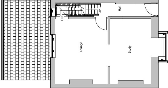
⑥ Existing Ground Floor 1 : 100
