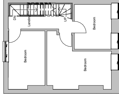
⑦ Existing First Floor 1 : 100
