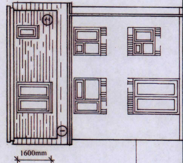
REAR ELEVATION (1:100)
