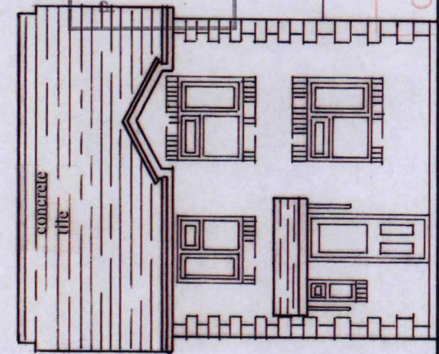
FRONT ELEVATION (1:100)
