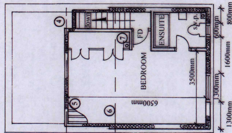
ATTIC PLAN (1:100)
