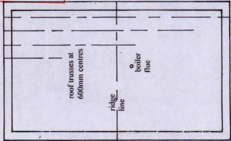
ATTIC PLAN (1:100)
