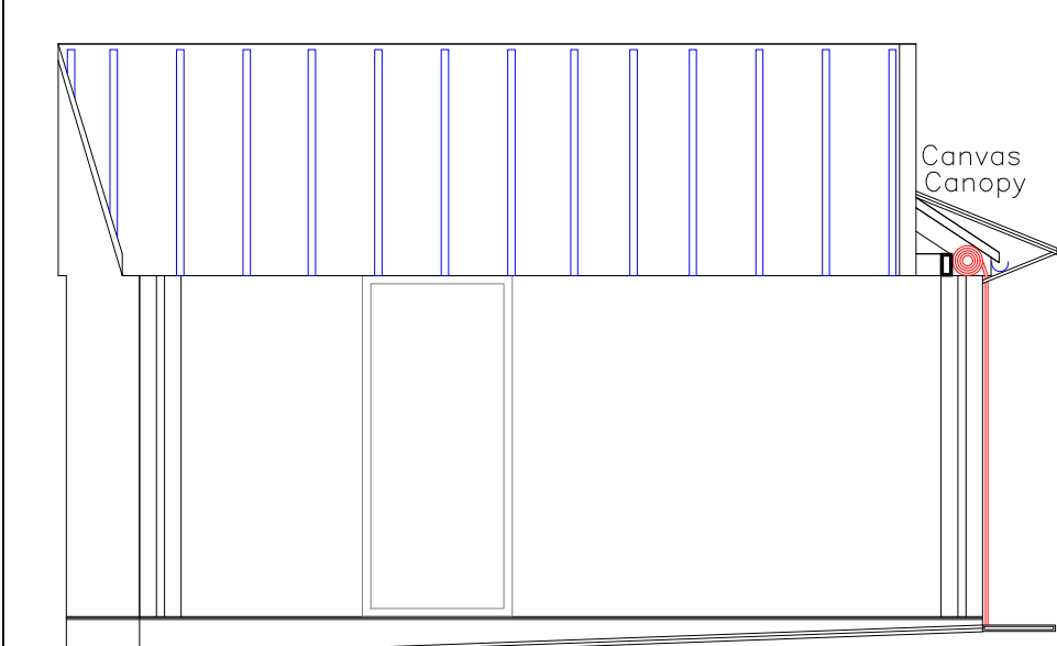
Proposed Section 1:50
