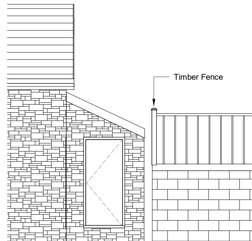
Bin Store East Elevation
