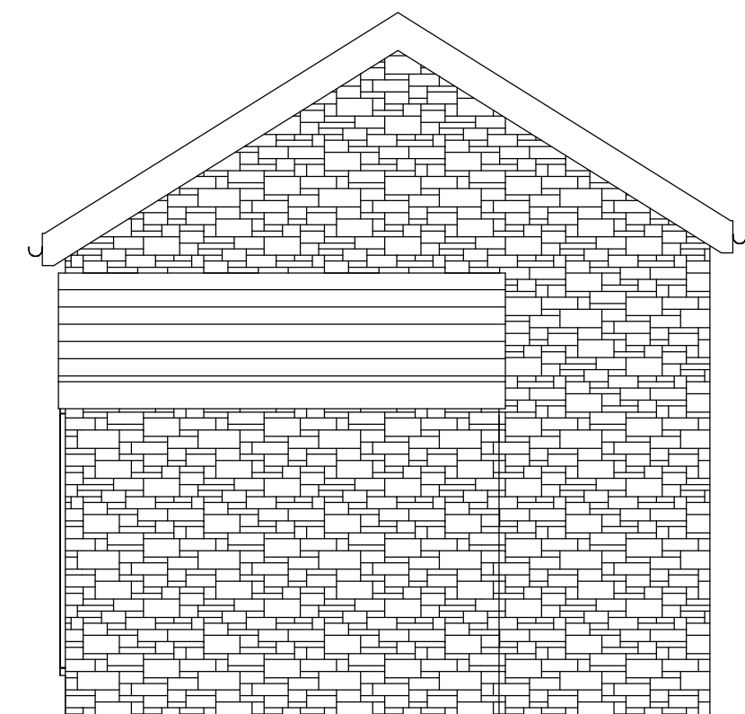
Bin Store Rear Elevation
