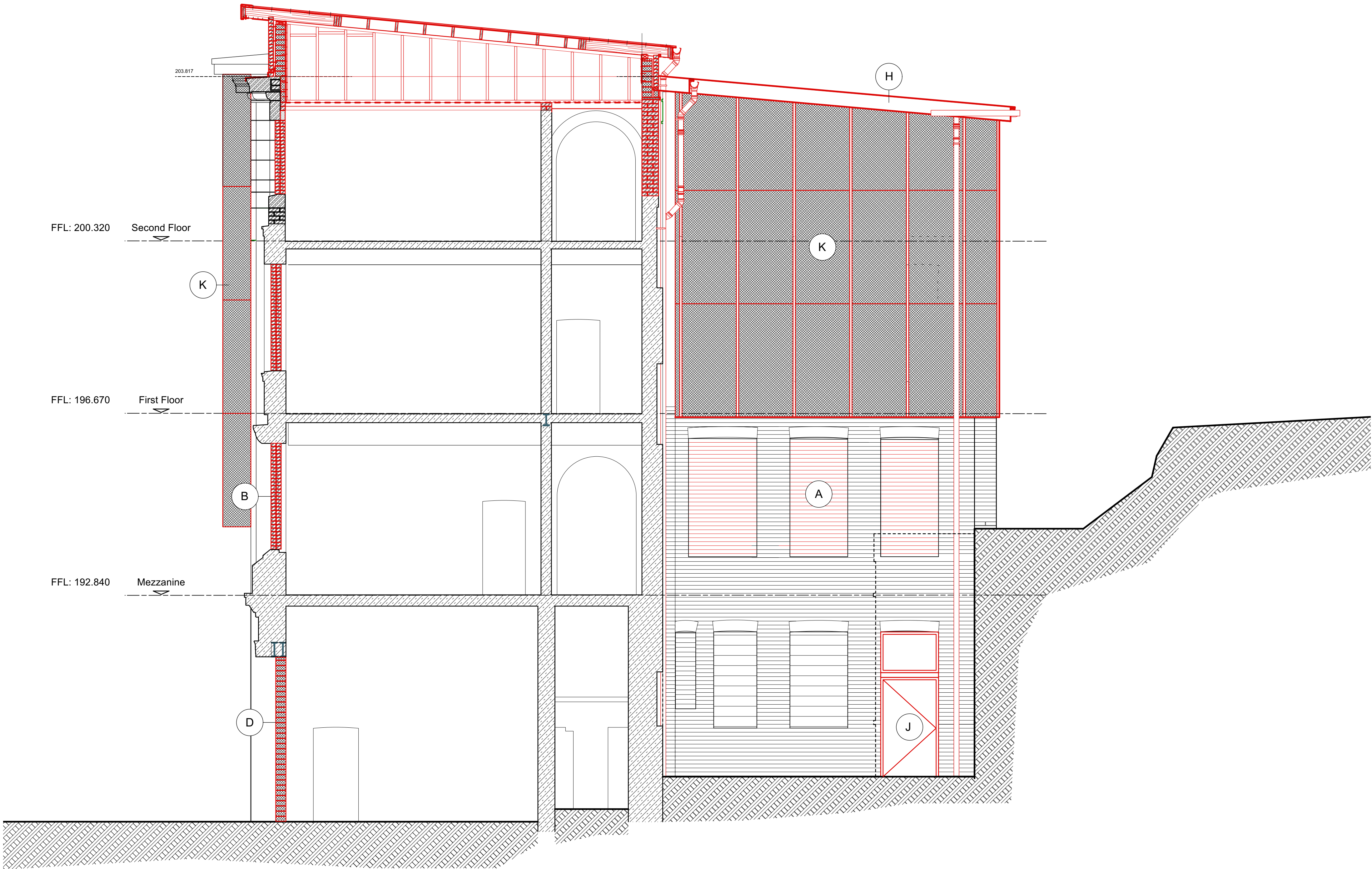
1 Proposed Narrow Section A-A Scale: 1:50
