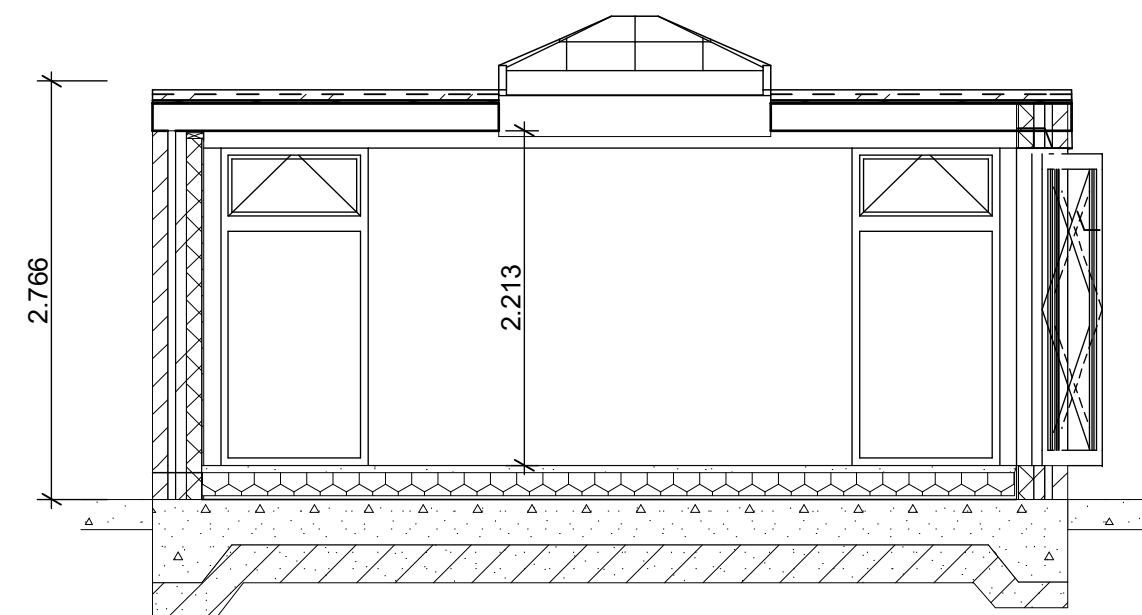
Building section S1. Scale 1:50
