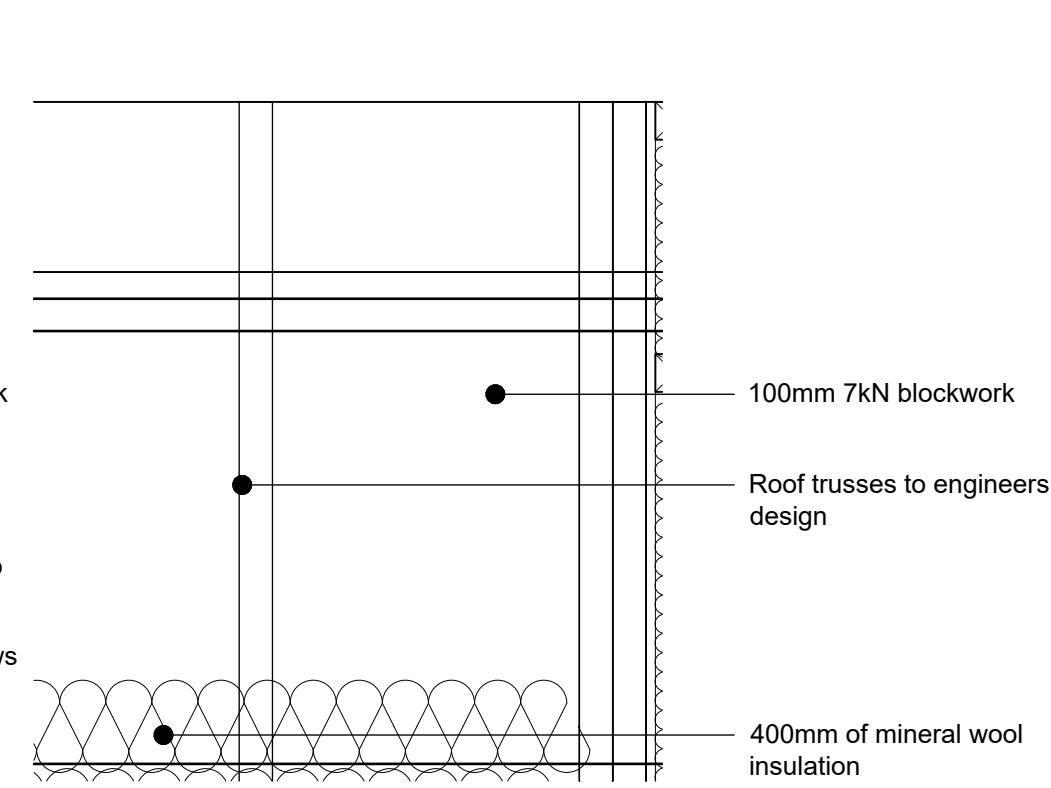
Detail 07 Scale 1:10
