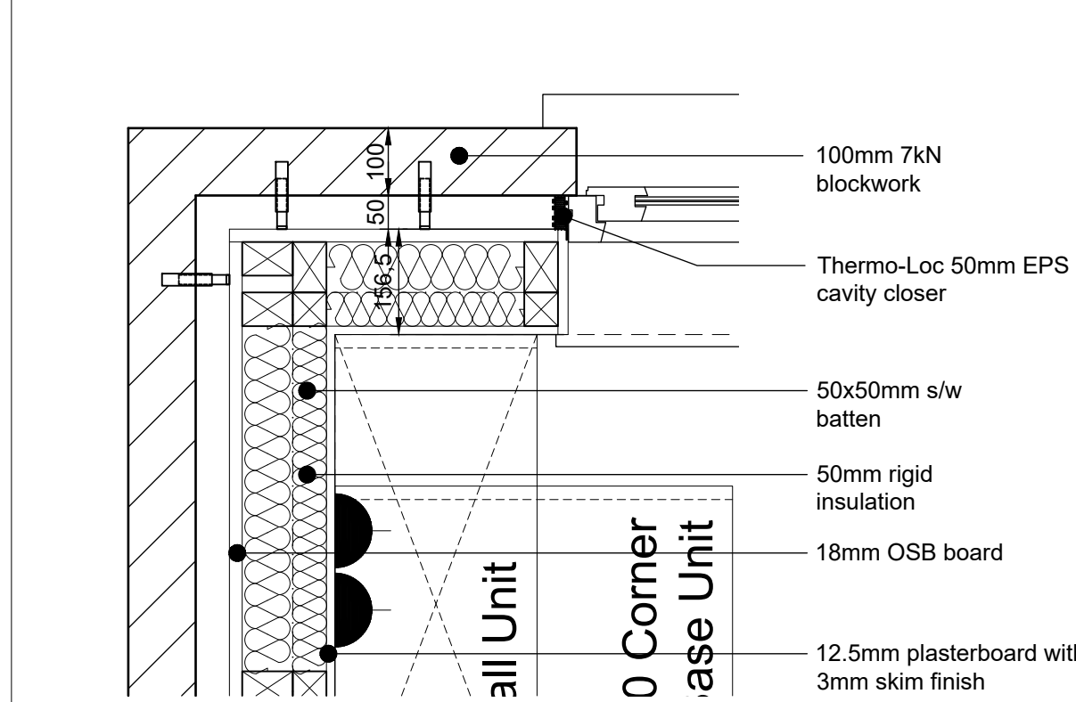
Detail 01 Scale 1:10
