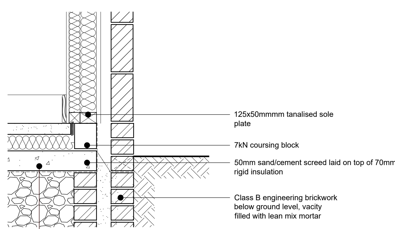
Detail 04 Scale 1:10
