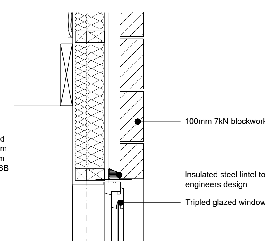
Detail 06 Scale 1:10
