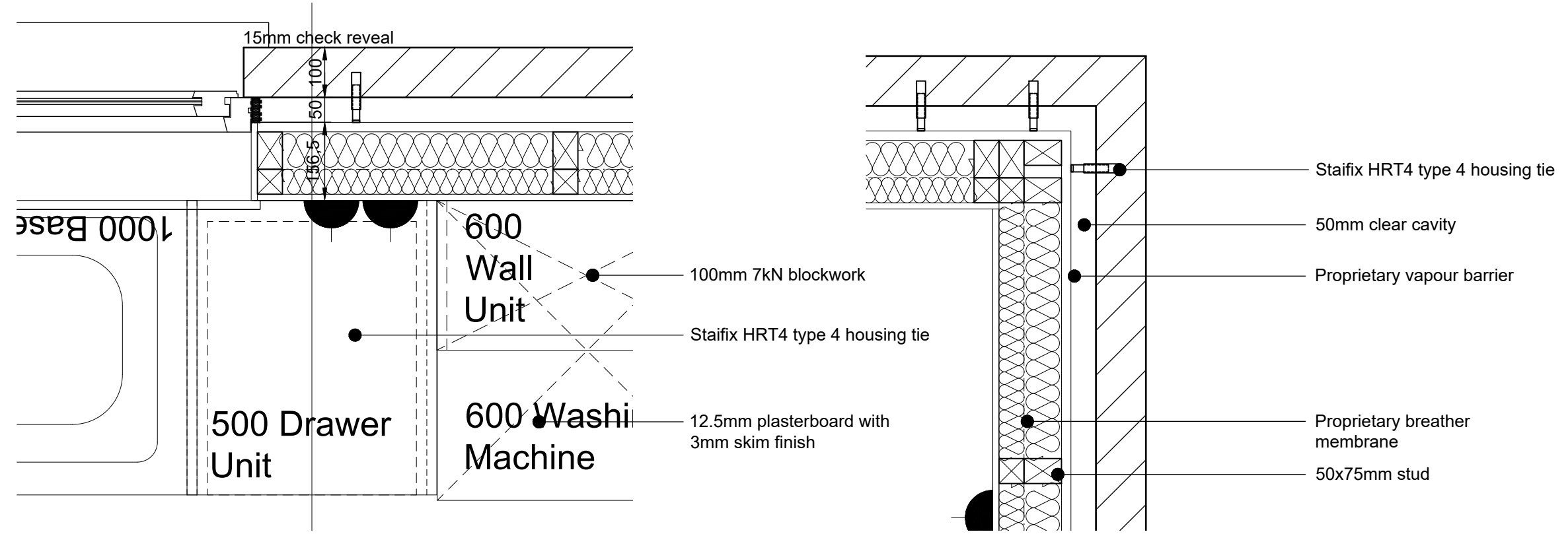
Detail 02 Scale 1:10
