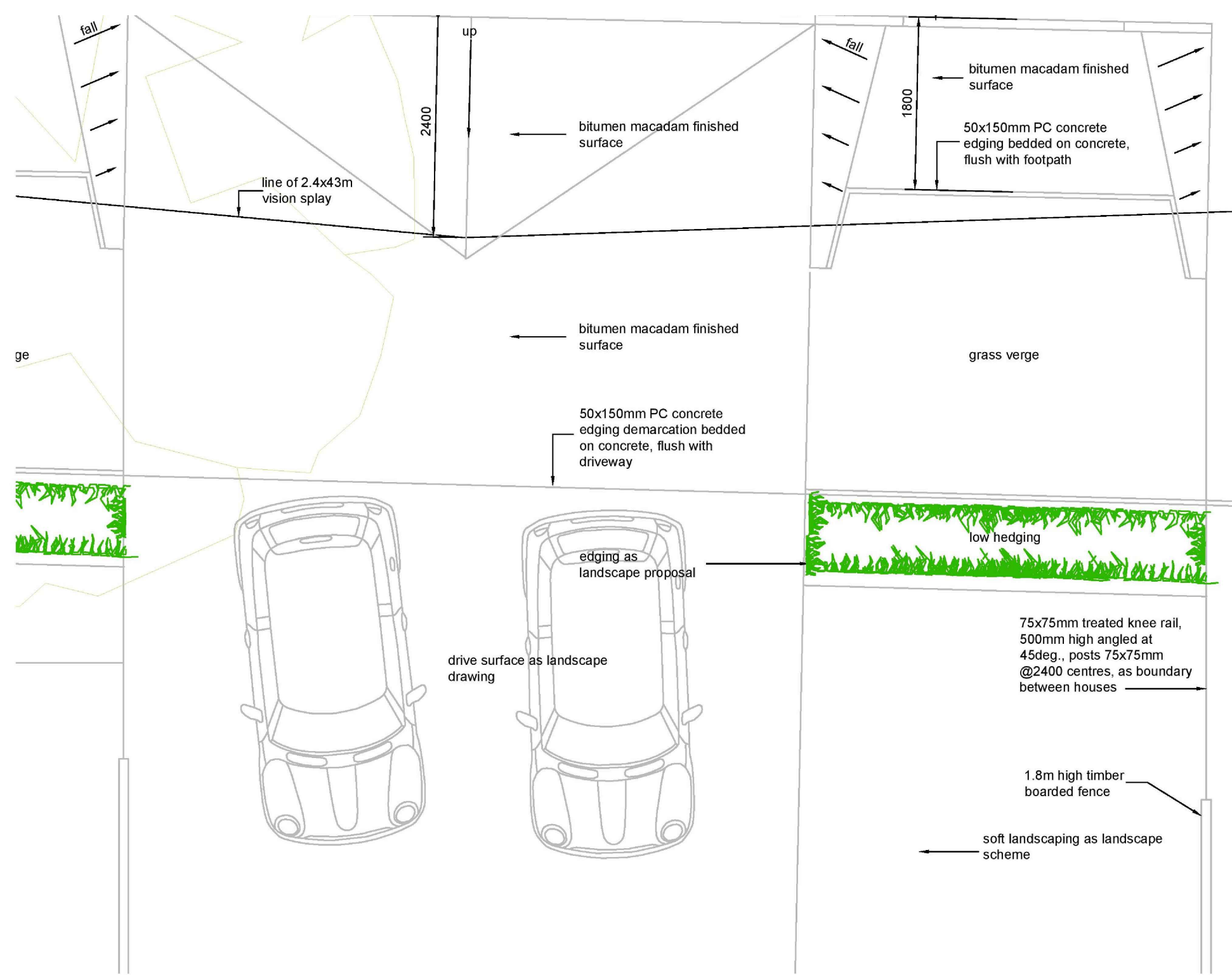
Typical Crossover/ Plan Scale 1:50
