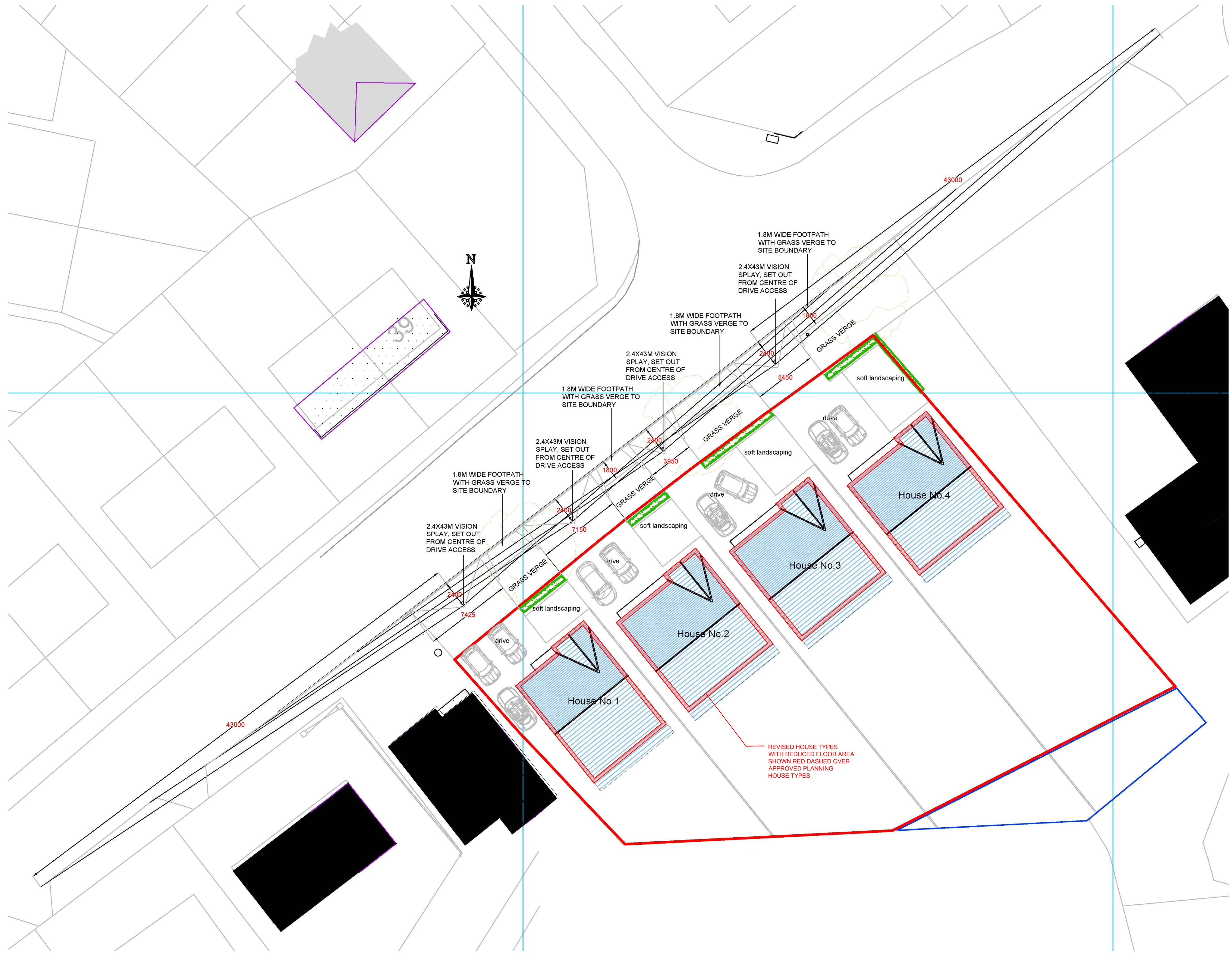
Vision Splay Plan Scale 1:200
