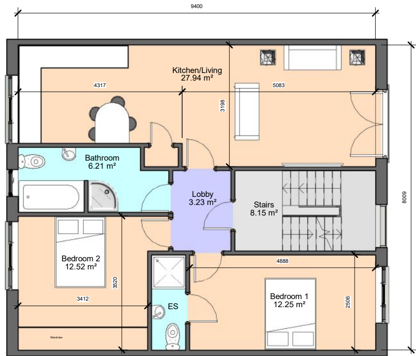
4 Third Floor
