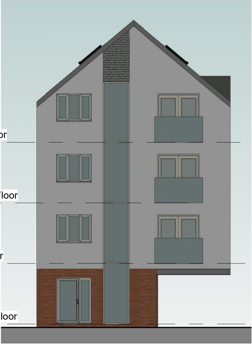
FRONT ELEVATION 1 : 100
