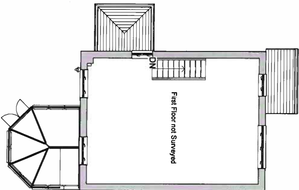
2 Existing First Floor 1 : 100
