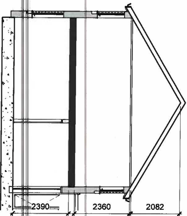
1 Existing Ground Floor 1 : 100
