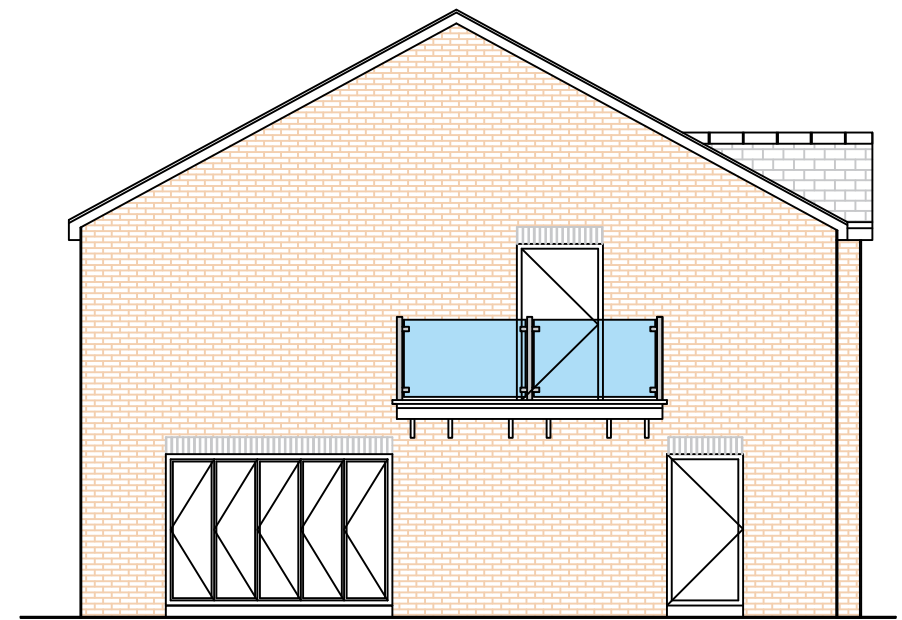
Proposed North Facing Elevation 1:100
