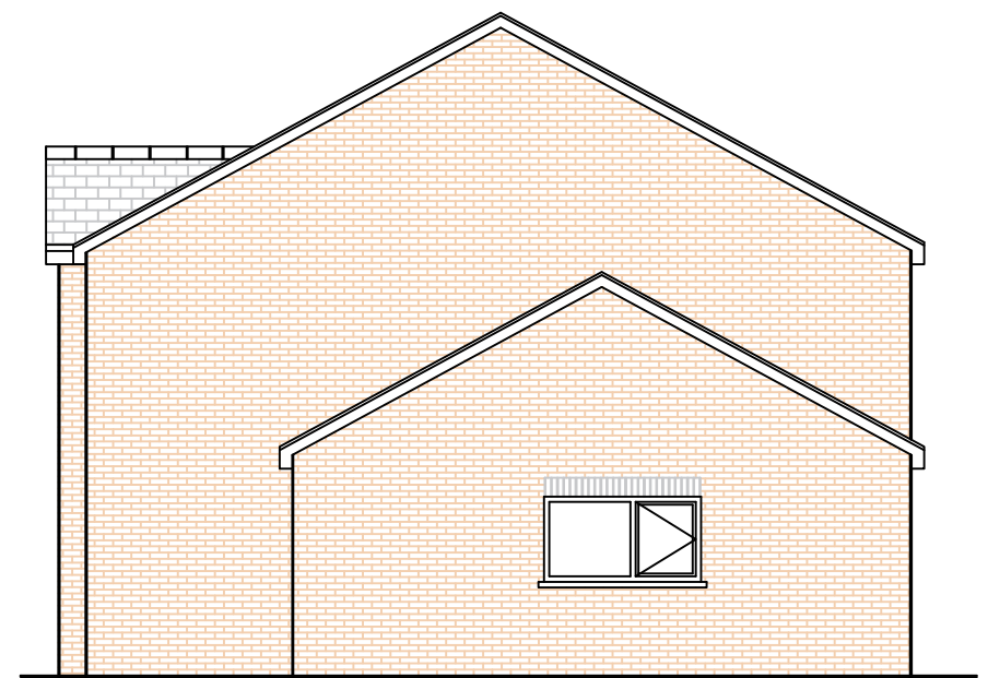
Proposed South Facing Elevation 1:100
