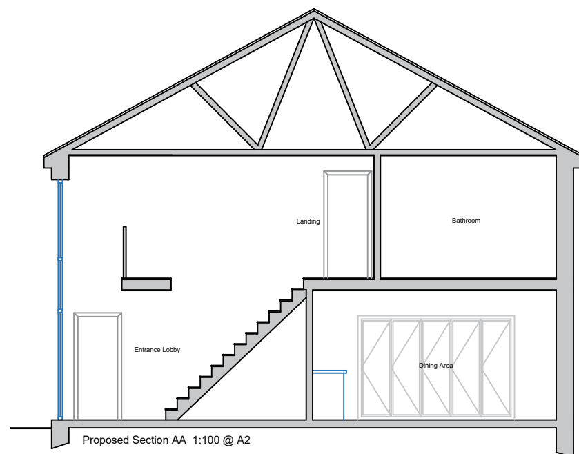
Proposed Section AA 1:100 @ A2
