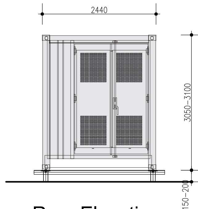
Rear Elevation
