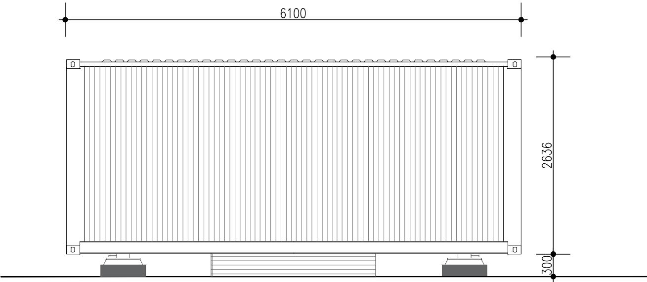
Rear Elevation
