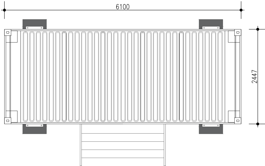
Roof Plan
