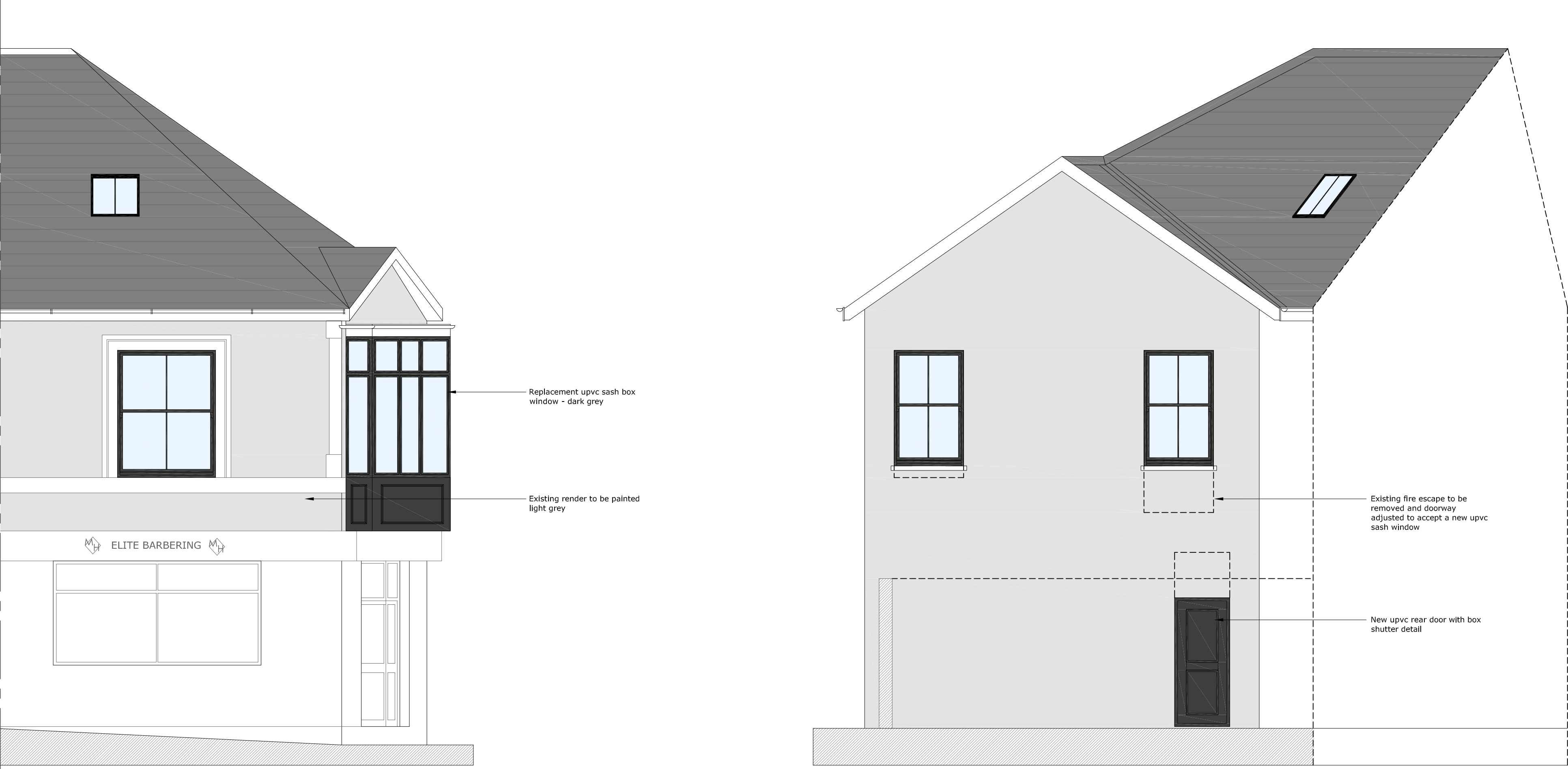
Front Elevation
