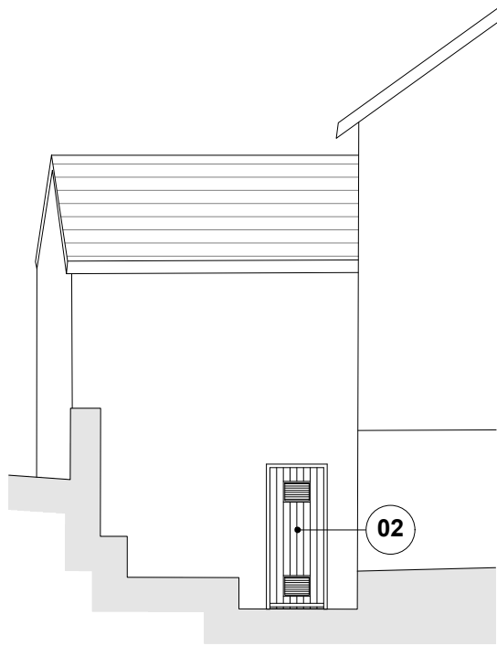
2 WEST ELEVATION (PART) AS PROPOSED 225 1:100 (approx)
