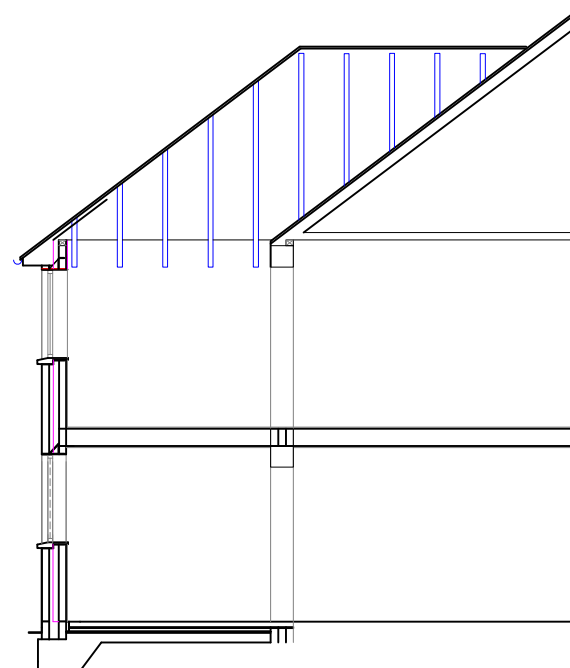
Proposed Section 1:100
