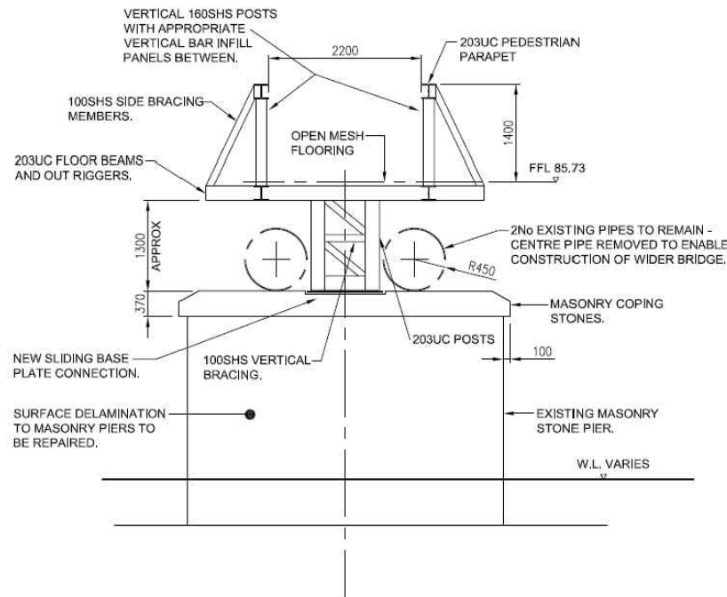
TYPICAL SECTION THROUGH BRIDGE.
