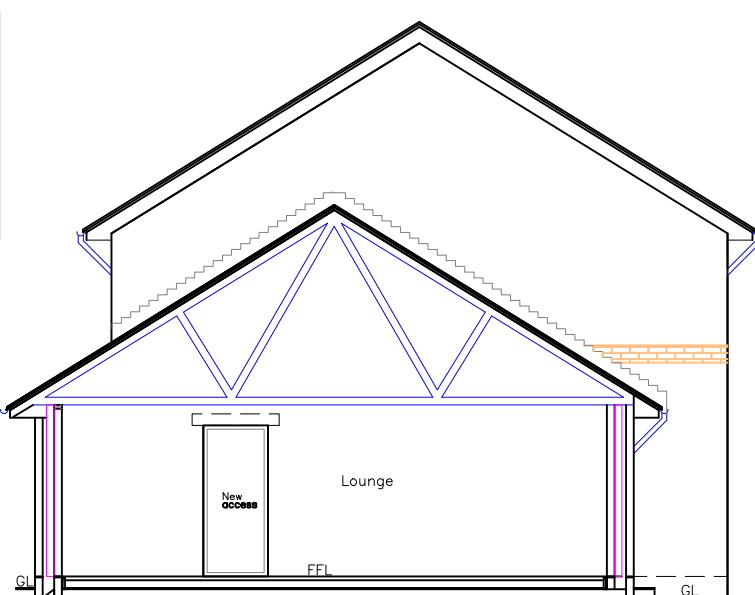
Proposed Section 1:100
