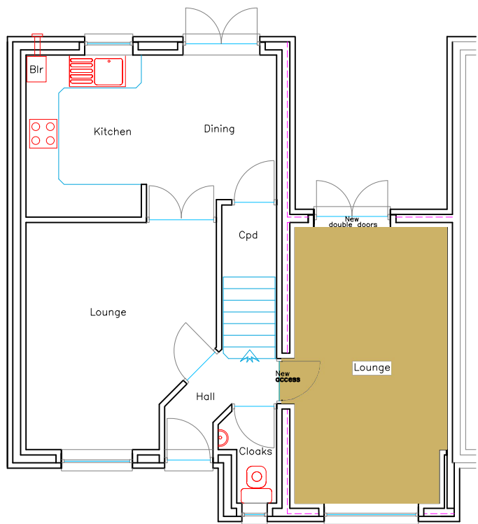
Proposed Floor Plan 1:100
