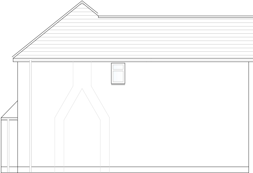
side SOUTH — WEST elevation
