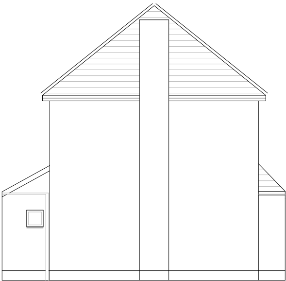
side NORTH — EAST elevation
