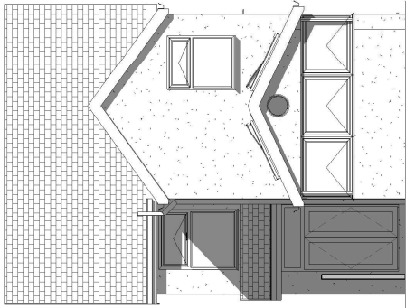
1 Existing Rear Elevation 1 : 100
