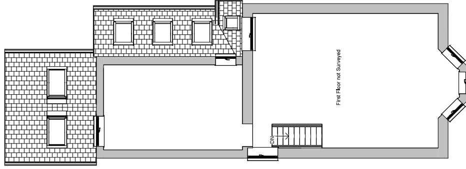
4 Proposed First Floor 1 : 100
