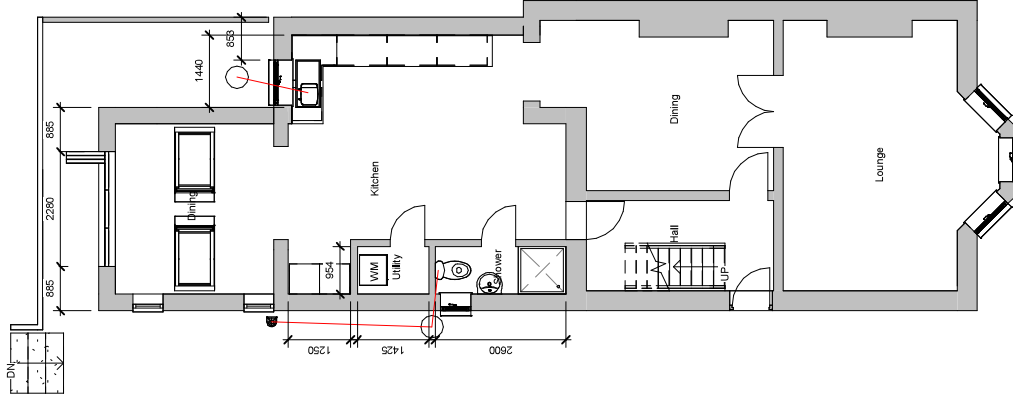
3 Proposed Ground Floor 1 : 100
