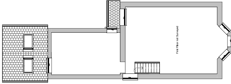
2 Existing First Floor 1 : 100
