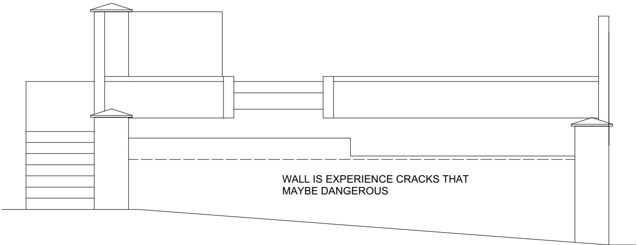
FRONT ELEVATION EXISTING
