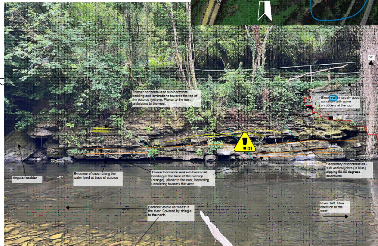
South Abutment (Wall) Elevation View
