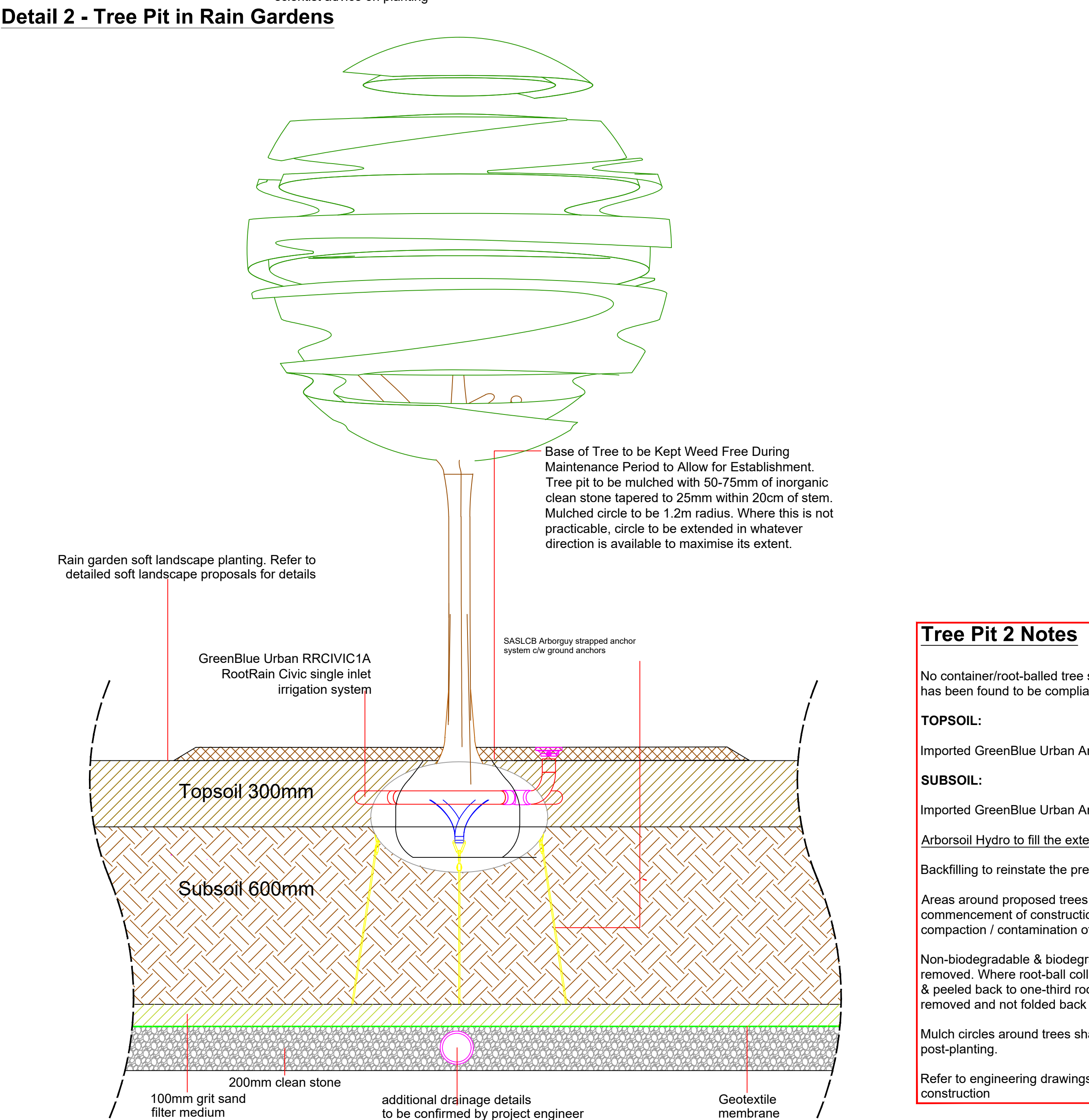
Detail 2 - Tree Pit in Rain Gardens
