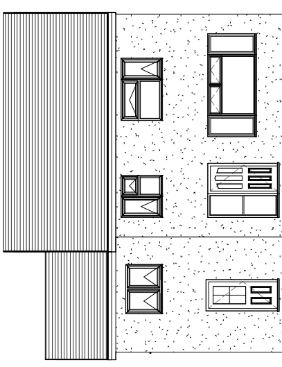
3 Proposed Front Elevation 1 : 100
