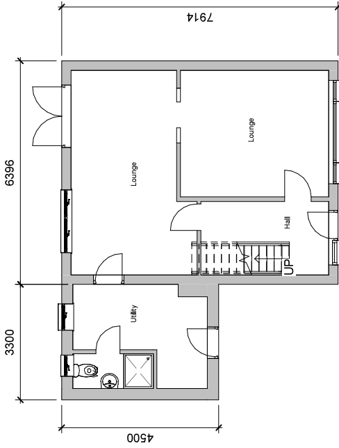
1 Proposed Ground Floor 1 : 100
