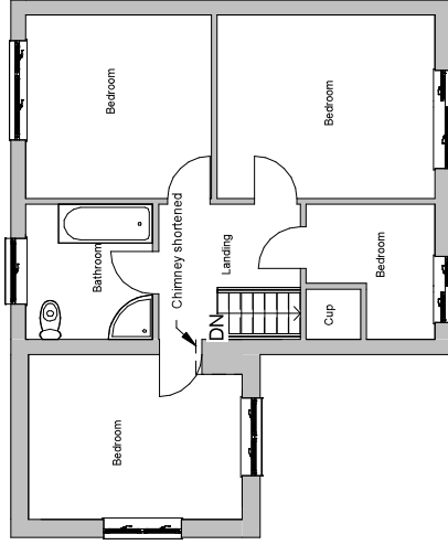
2 Proposed First Floor 1 : 100
