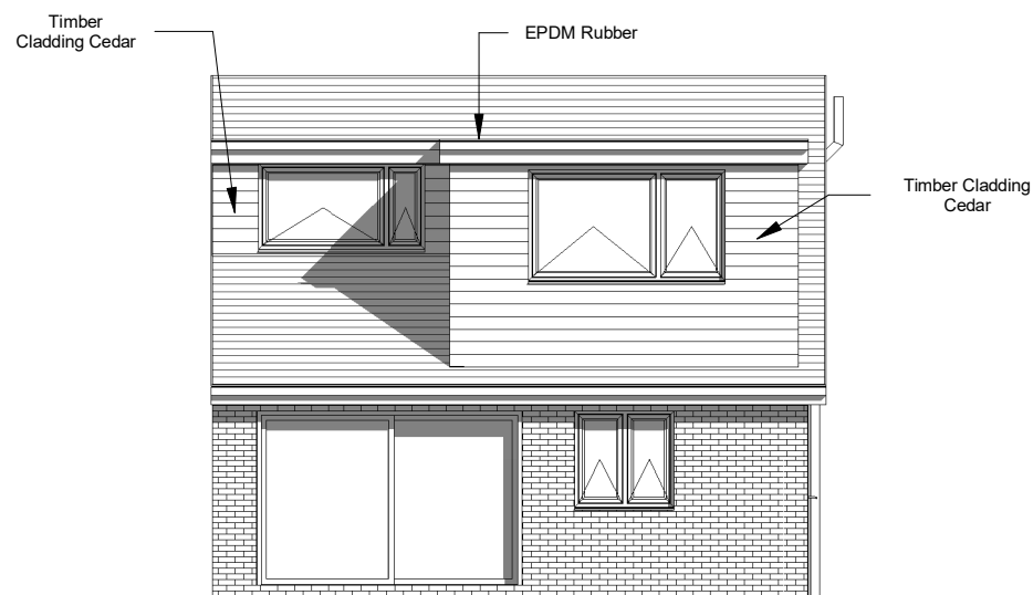
2 Proposed Rear Elevation 1 : 100
