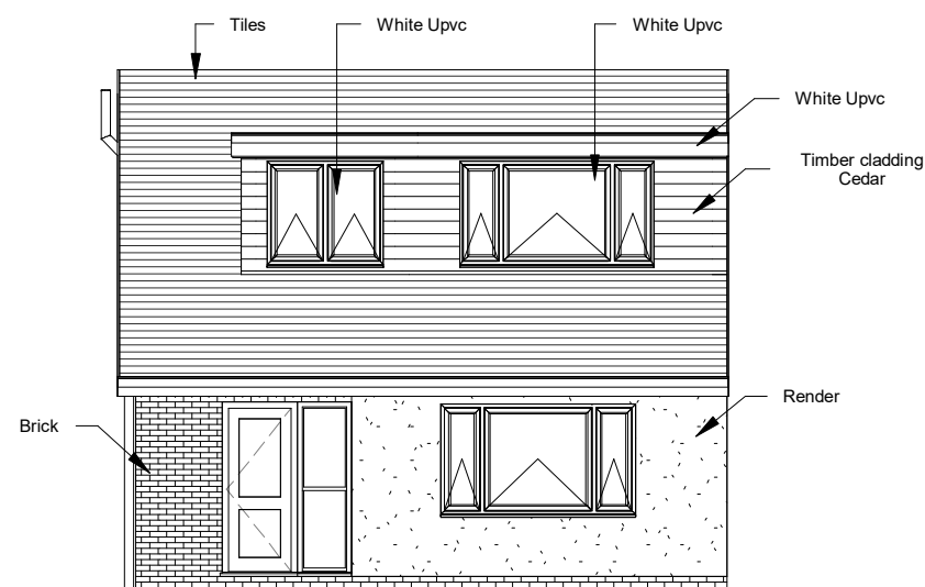
1 Proposed Front Elevation 1 : 100
