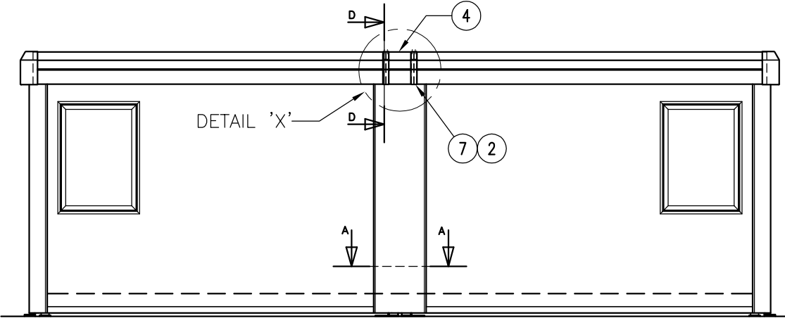
TYPICAL END ELEVATION OF MODULES
