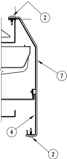
SECTION 'D-D'
