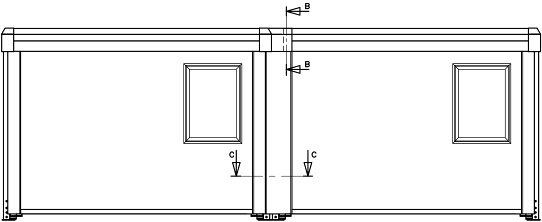
TYPICAL END ELEVATION OF OFFSET MODULES
