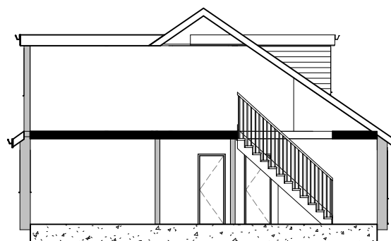
4 Proposed Section 1 : 100
