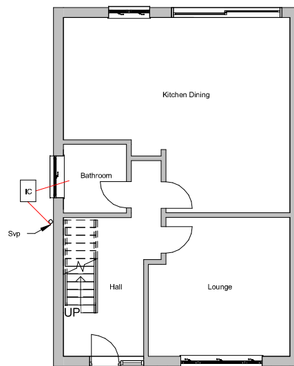
1 Proposed Ground Floor 1 : 100
