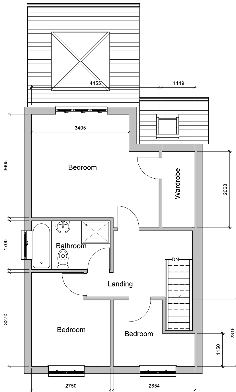
1 Proposed First Floor 1 : 50
