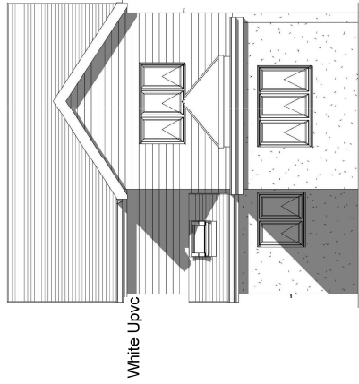
2 Proposed Rear Elevation 1 : 100
