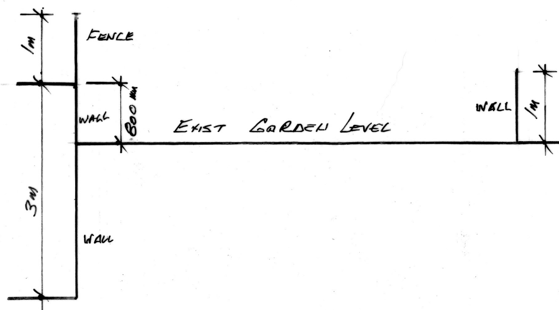
EXIST CROSS SECT. C 1
