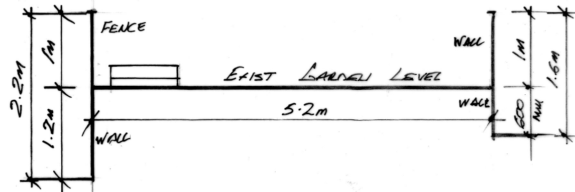
EXIST CROSS SECT. B 1
