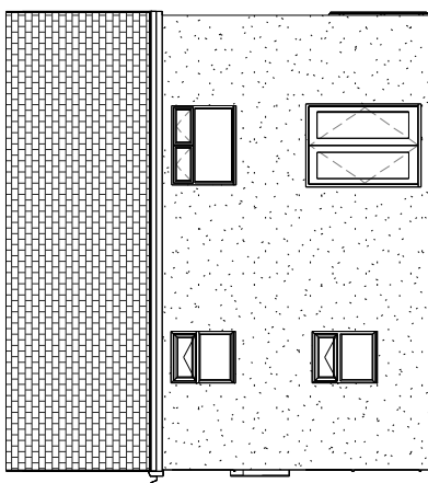
1 Proposed Front Elevation 1 : 100
