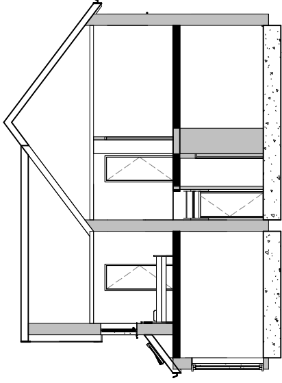
5 Proposed Section 1 : 100
