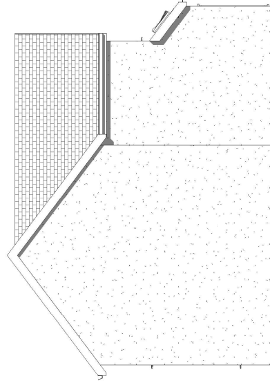
4 Proposed Side 2 Elevation 1 : 100
