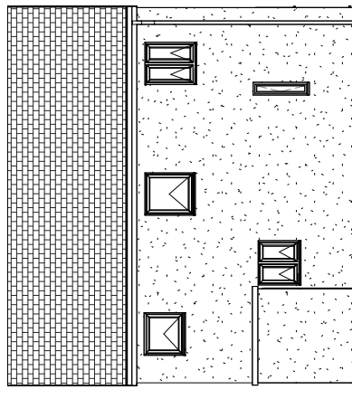
4 Existing Rear Elevation 1 : 100
