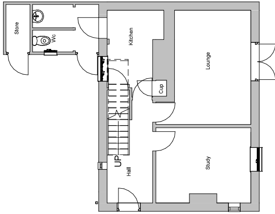
1 Existing Ground Floor 1 : 100
