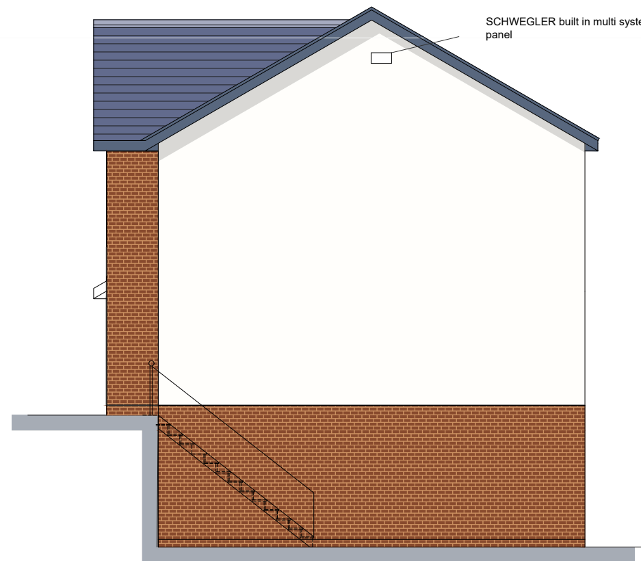
PROPOSED SIDE ELEVATION - PLOT 1
