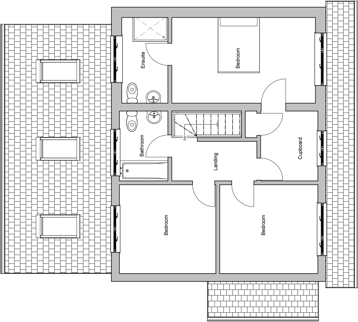
1 Proposed First Floor 1 : 50
