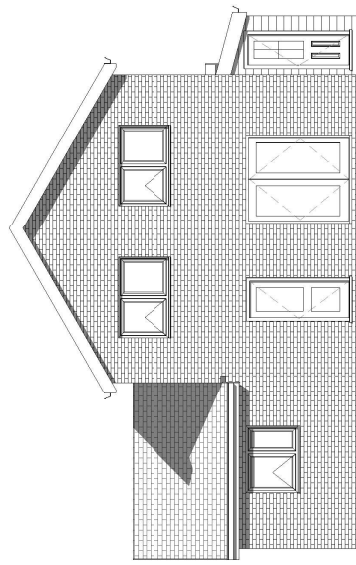
4 Existing Rear Elevation 1 : 100
