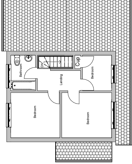
2 Existing First Floor 1 : 100
