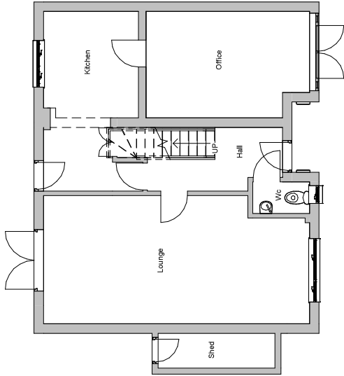
1 Existing Ground Floor 1 : 100
