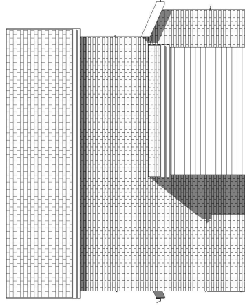
5 Existing Side 1 Elevation 1 : 100
