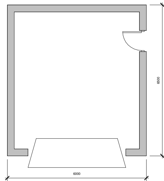
Ground Floor Plan - 1:100 @ A3
