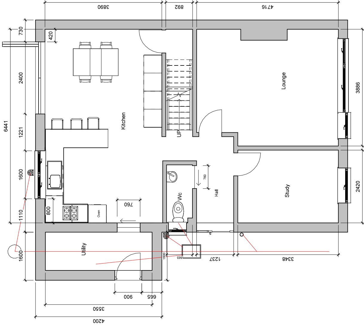
1 Proposed Ground Floor 1 : 50
