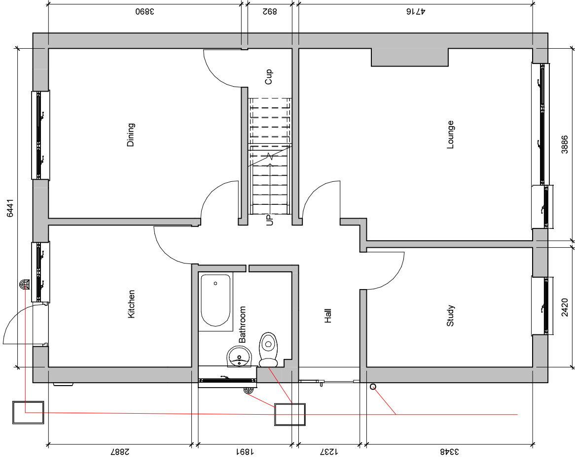
1 Existing Ground Floor 1 : 50
