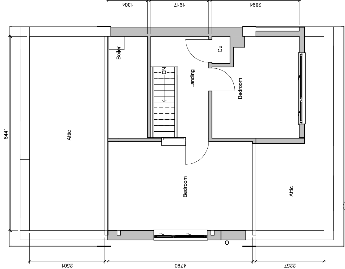
2 Existing First Floor 1 : 50
