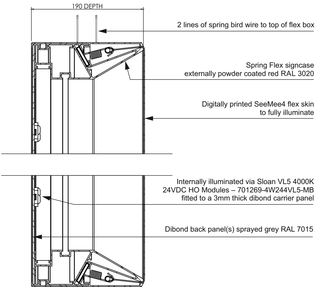
Example: Spring bird wire to top of flex box
