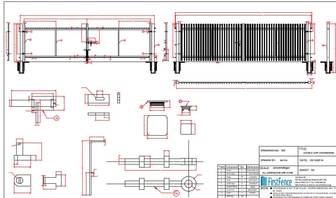
Detail B - Gate Specification
