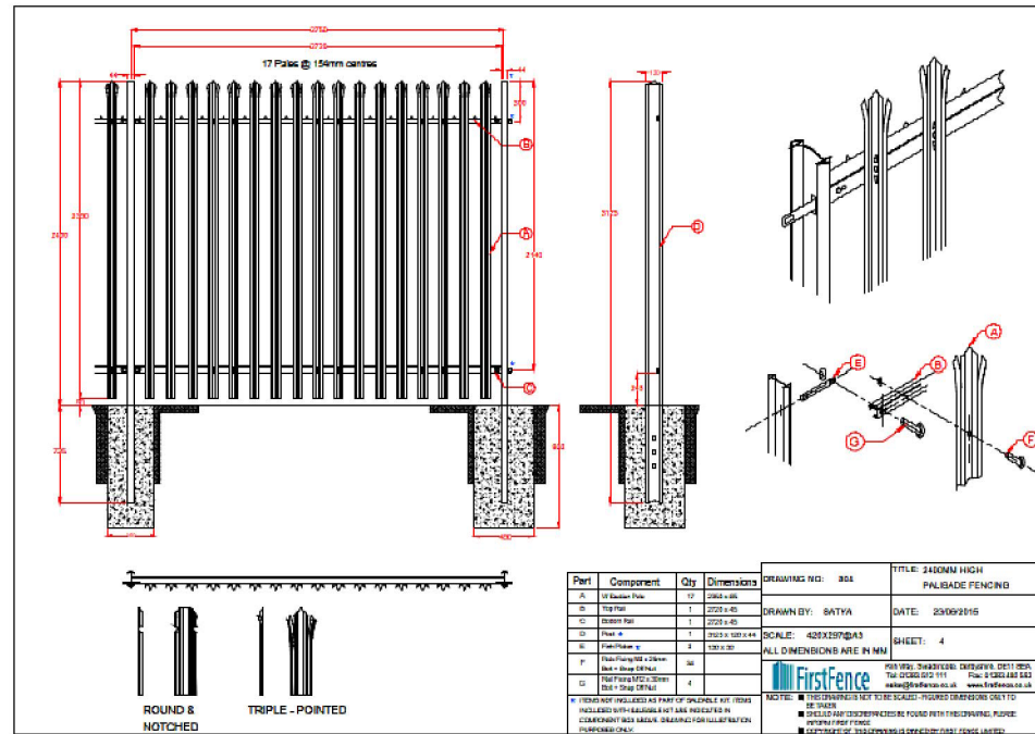
Detail A - Fencing Specification
