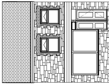
4 Proposed Front Elevation 1 : 100
