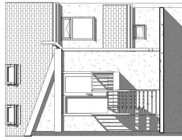
4 Existing Rear Elevation 1 : 100
