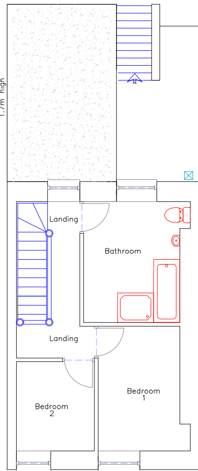
Proposed First Floor 1:100
