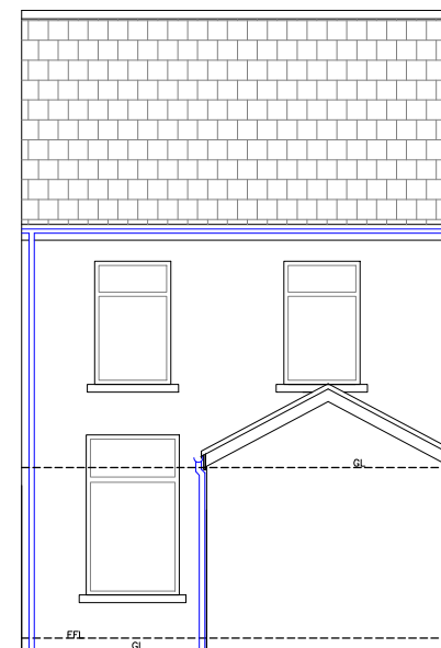
Existing Rear Elev 1:100
