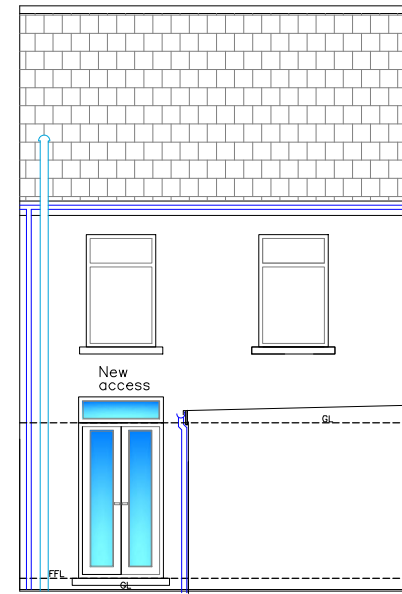
Proposed Rear Elev 1:100
