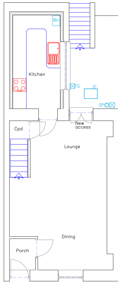
Proposed Ground Floor 1:100
