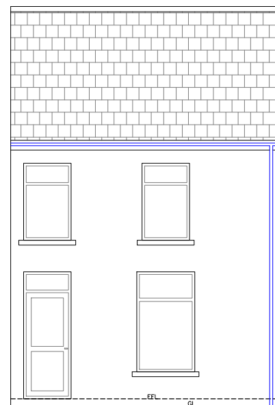
Existing Front Elev 1:100
