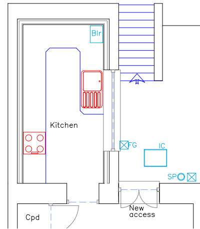
Proposed Ground Floor 1:50
