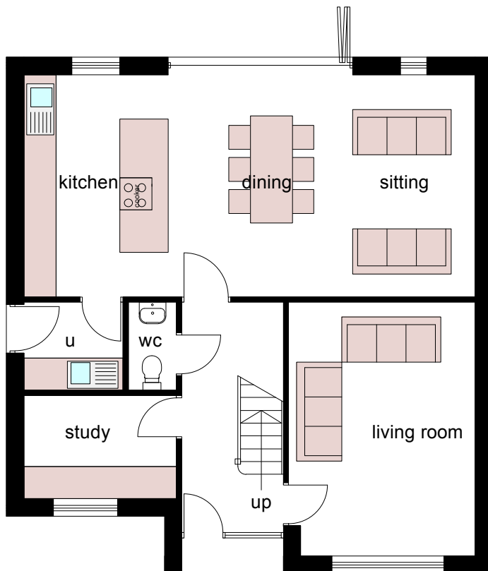
GROUND FLOOR PLAN - 72sqm
