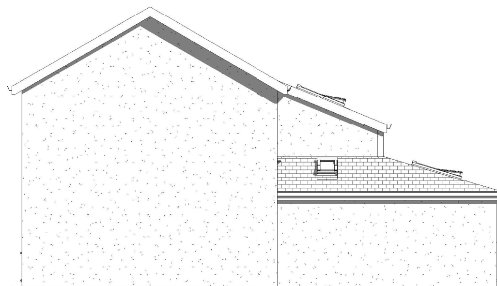
6 Proposed Side 2 Elevation 1 : 100
