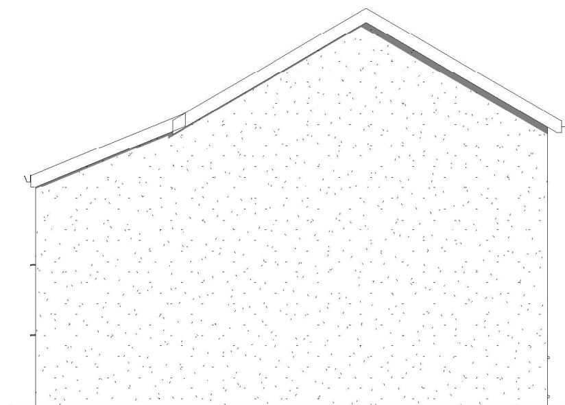
5 Existing Side 1 Elevation 1 : 100
