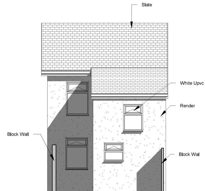
4 Existing Rear Elevation 1 : 100
