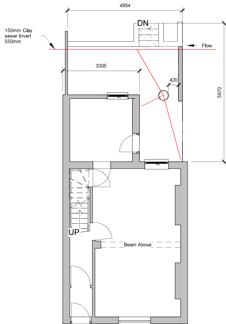
1 Existing Ground Floor 1 : 100
