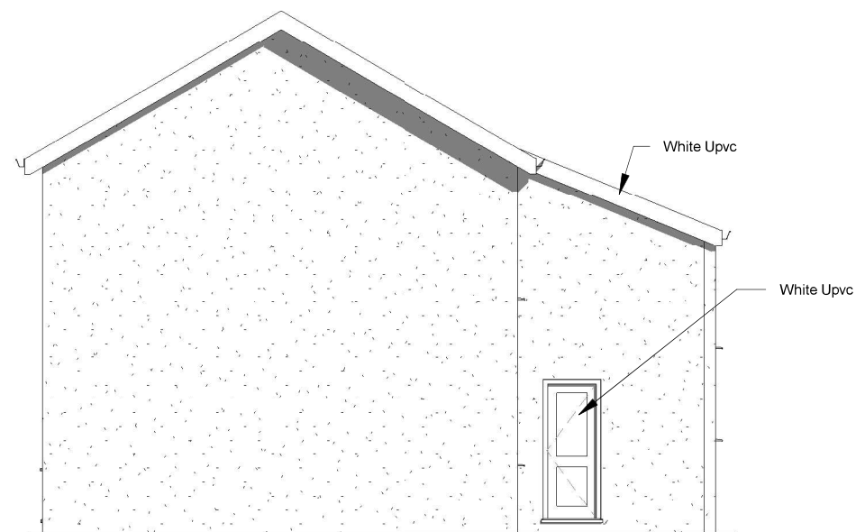
6 Existing Side 2 Elevation 1 : 100
